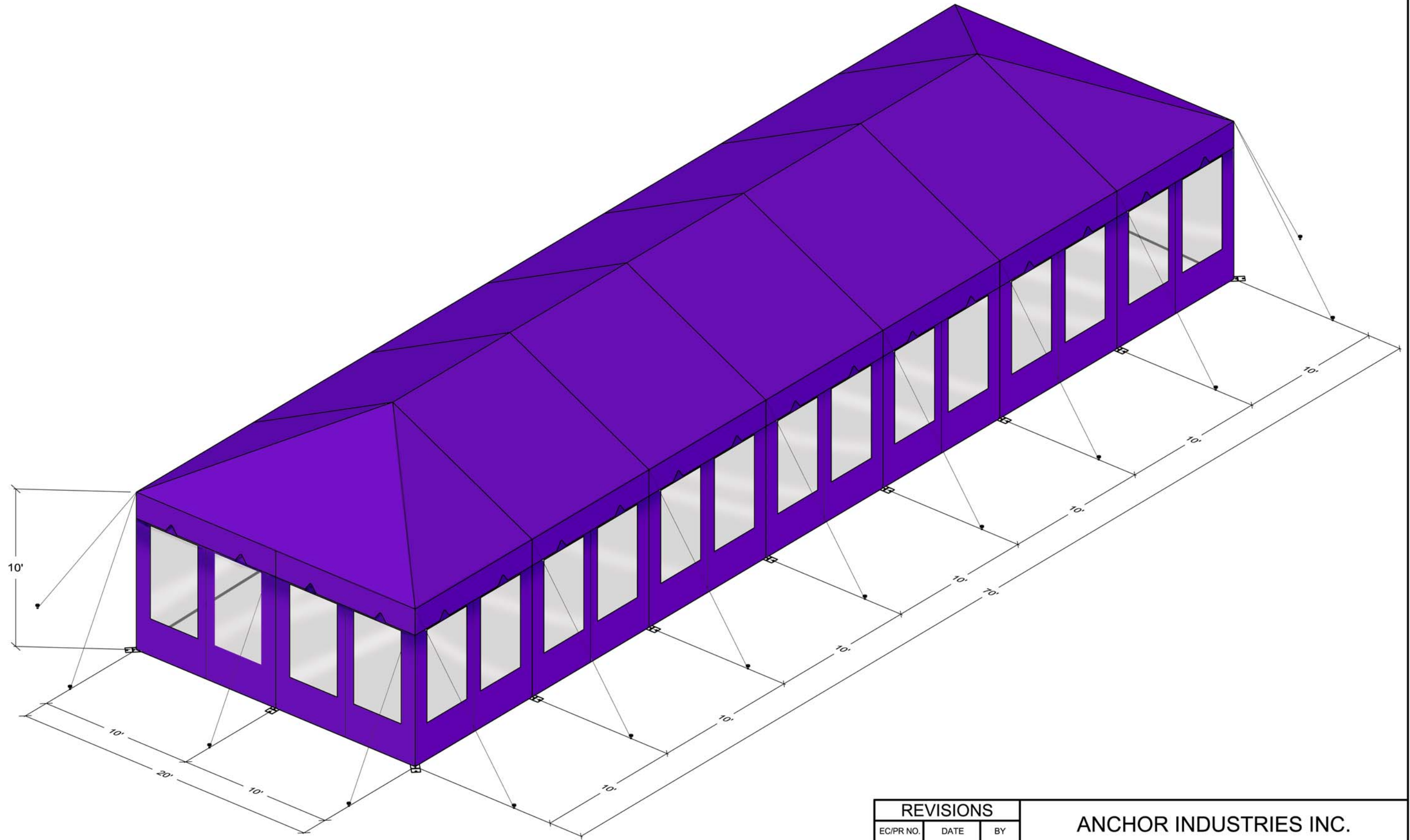
ISOMETRIC VIEW
